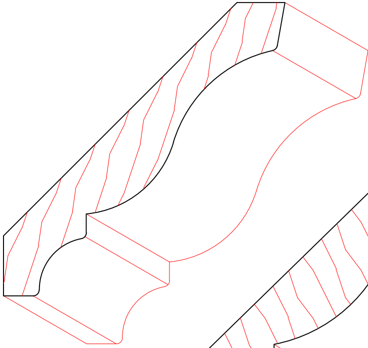
TM3066 3/4" X 4-1/4"
