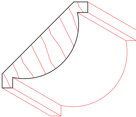
TM3030 5/8" X 2-3/16"
