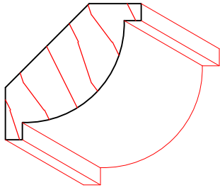
TM3153 1/2" X 1-7/16"
