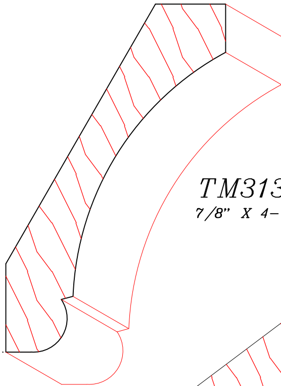
TM3138 3/4" X 5-1/8"
