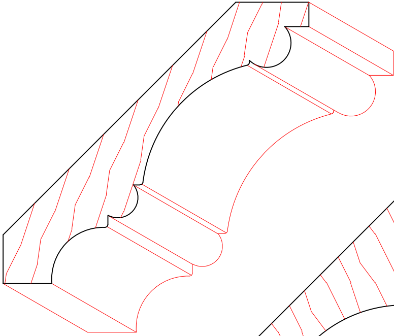
TM3037 3/4" X 4-3/16"
