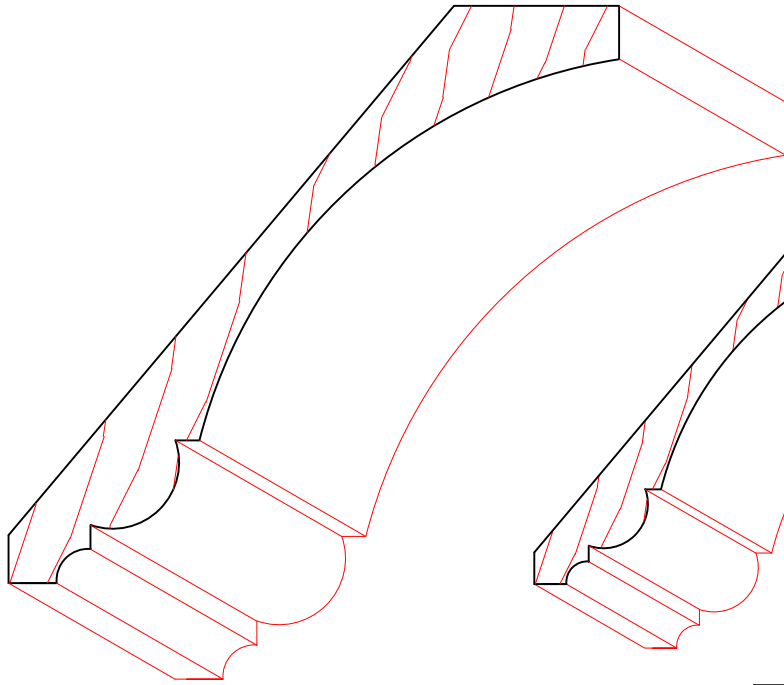
TM3004 13/16" X 4-3/8"
