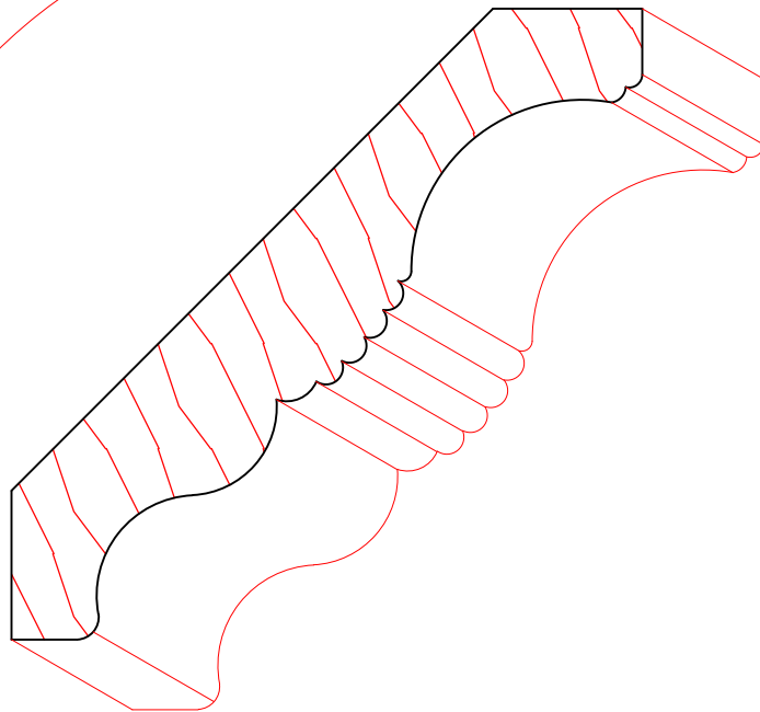
TM3183 3/4" X 4-1/4"
