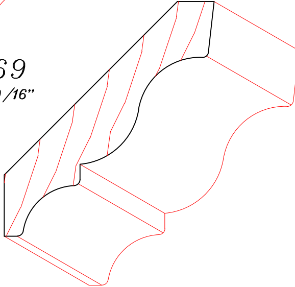
TM3070 3/4" X 3-3/16"
