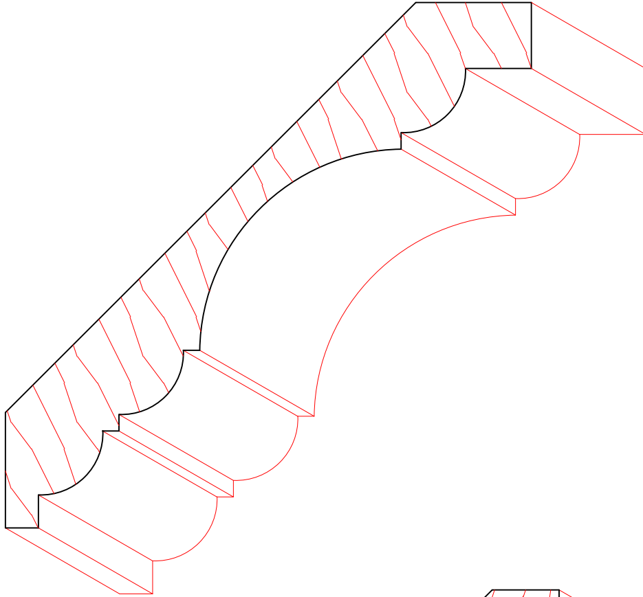
TM3087 7/8" X 5-5/8"
