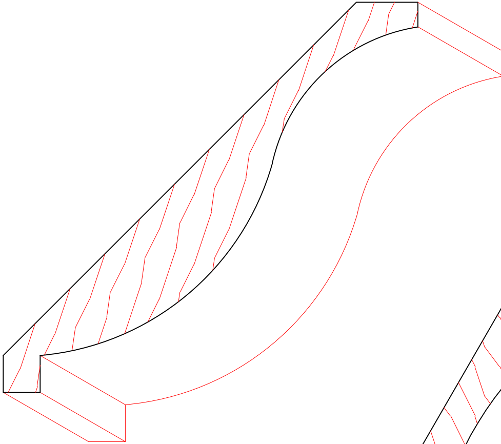
TM3047 7/8" X 5-13/16"
