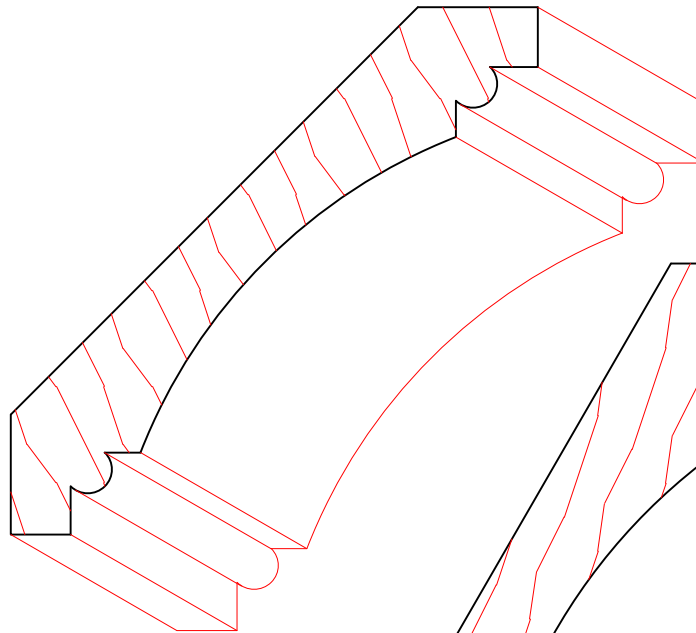
TM3005 11/16" X 3-7/8"
