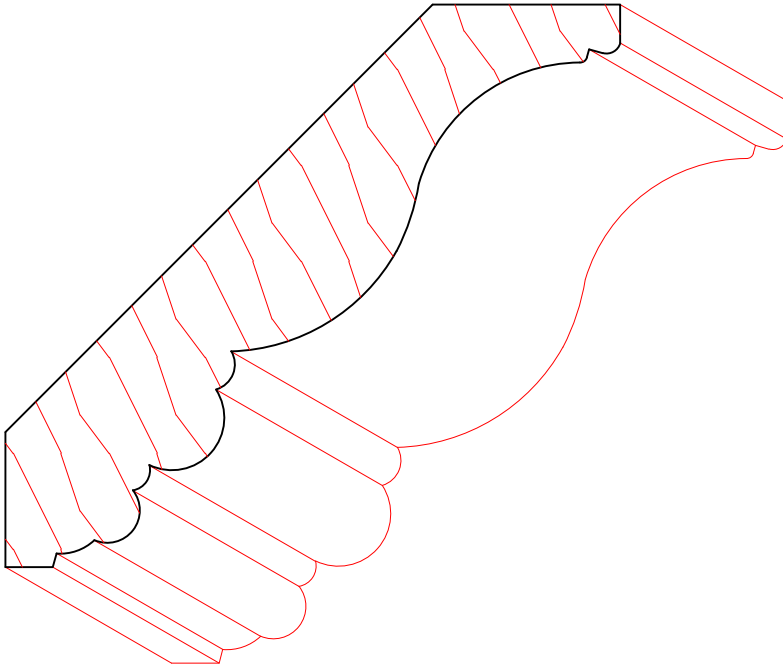
TM3034 13/16" X 4-5/16"
