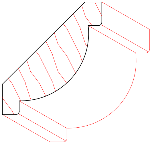
TM3054 13/16" X 2-3/4"
