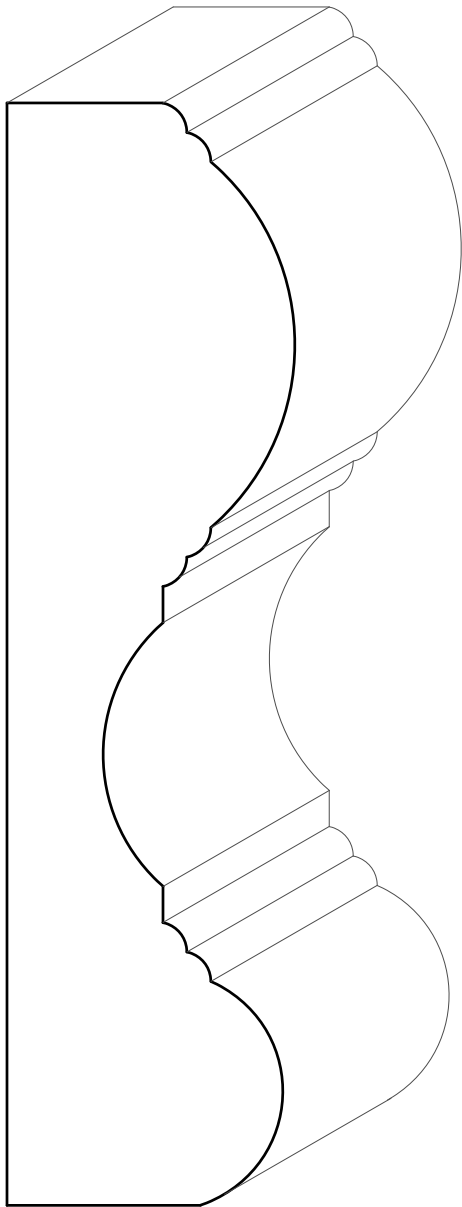
TM6001 1-1/2" X 5-3/4"
