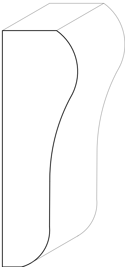
TM6082 1-3/8" X 4-5/16"
