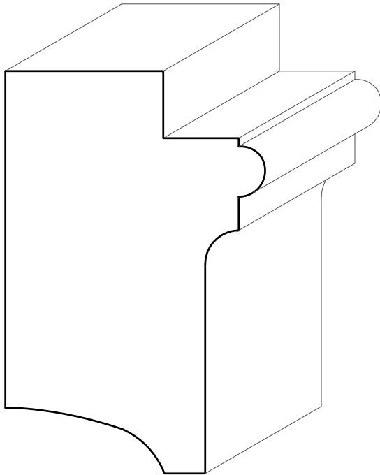
TM6058 1-15/16'' \times 3''
