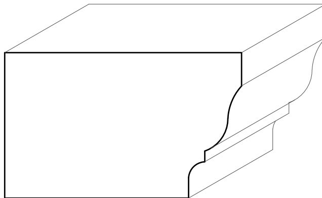
TM6046 1-1/2" X 2-7/16"
