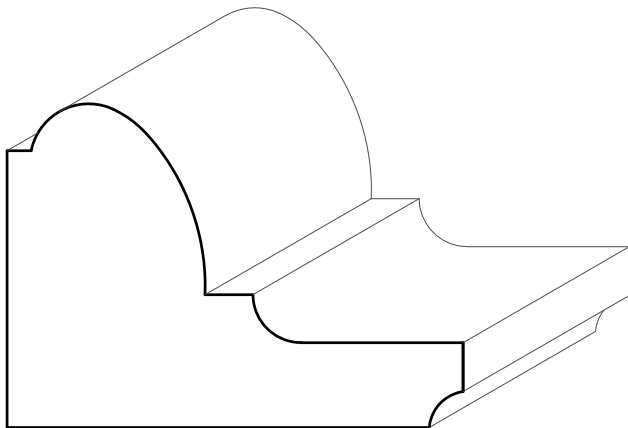
TM6060 1-11/16'' \times 2-3/8''
