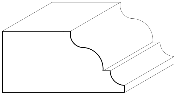
TM6007 1-1/16" X 2-1/8"
