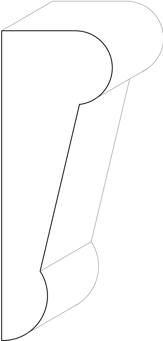
TM6070 1-7/8'' \times 5-1/4''
