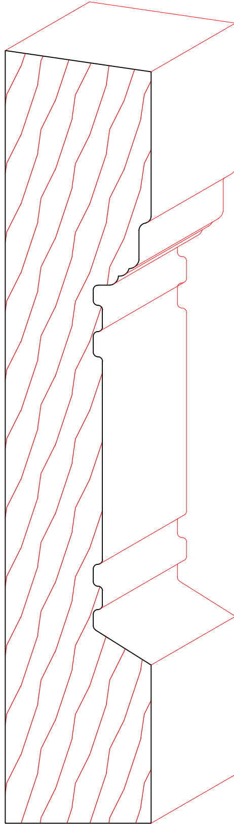
TM6078 1-1/2" X 7-15/16"
