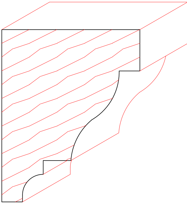
TM6047 2-1/2" x 3-1/8"
