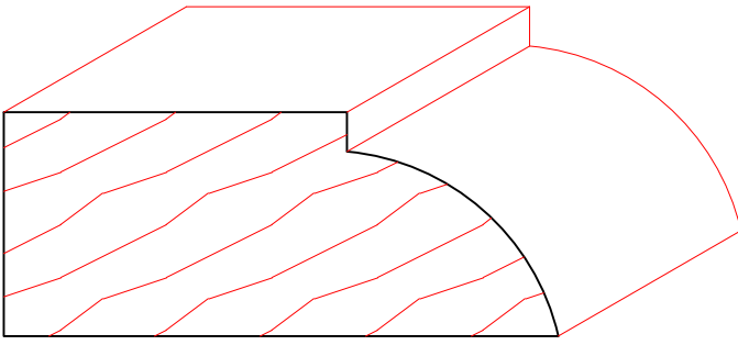
TM6018 1-1/16" X 2-5/8" +-
