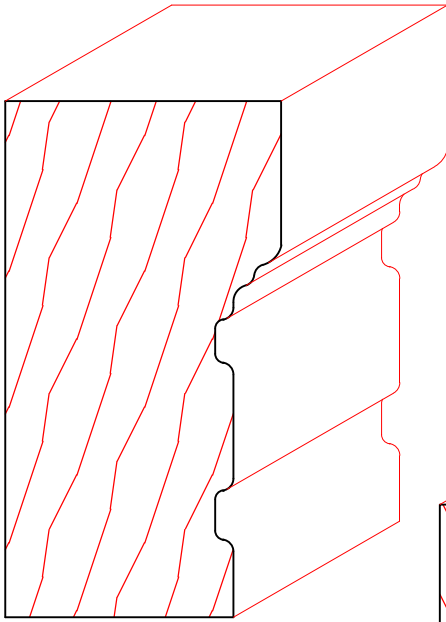
TM6079 1-7/16" X 2-11/16"
