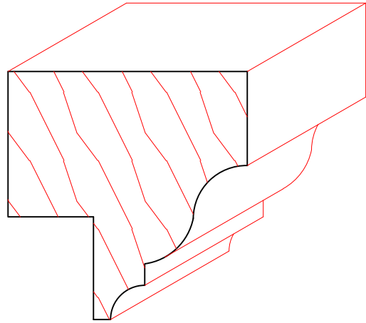
TM6049 1-3/4" x 1-13/16"
