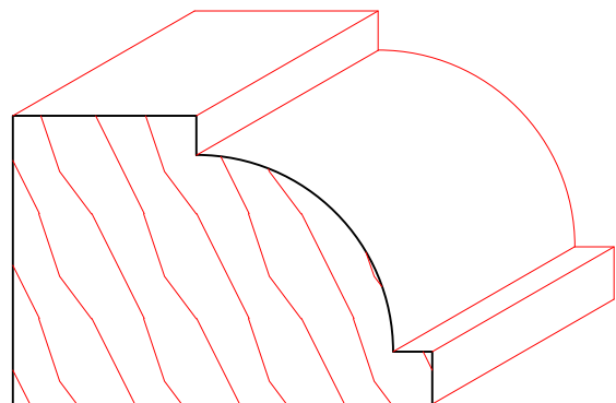
TM6009 1-3/8" X 2"
