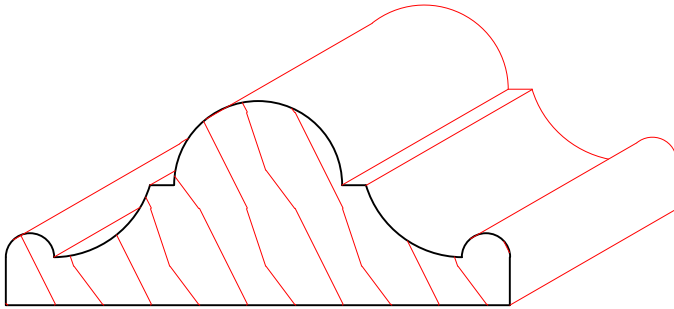
TM6020 1-1/16" X 2-5/8"
