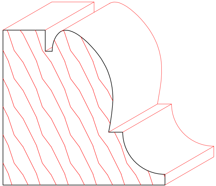
TM6057 2-3/4" X 2-7/8"
