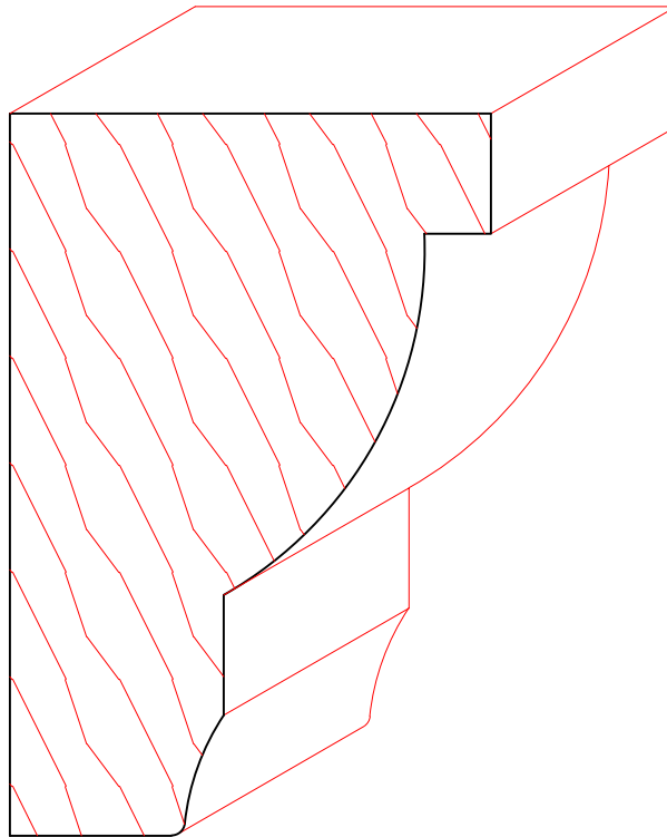
TM6031 2-1/4" X 3-3/8"
