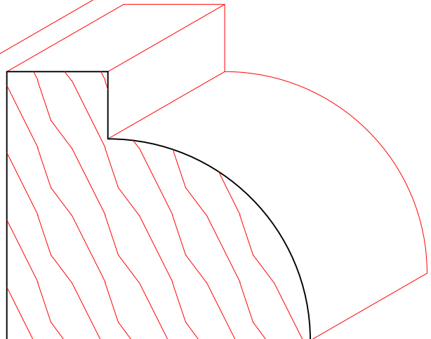
TM6016 1-3/4" X 3-1/2"
