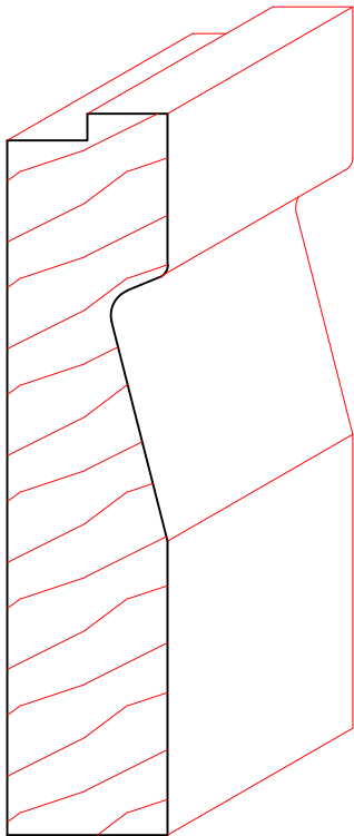
TM6045 3/4" x 3-3/8"
