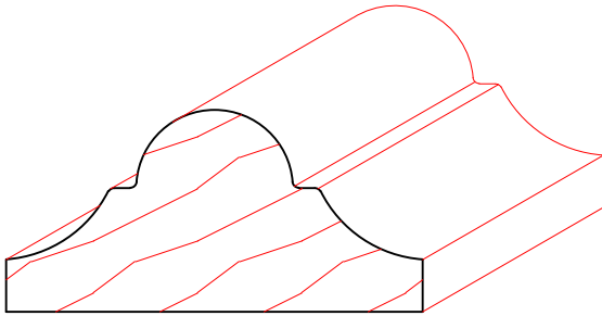
TM6020 1-1/16" X 2-5/8"
