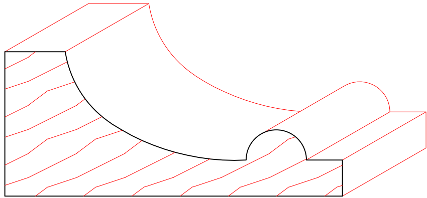
TM6032 1-1/2" X 3-1/2"
