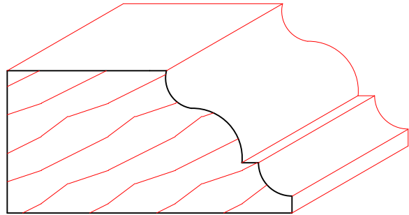
TM6007 1-1/16" X 2-1/8"
