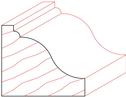
TM6039 1-1/2" X 1-3/4"
