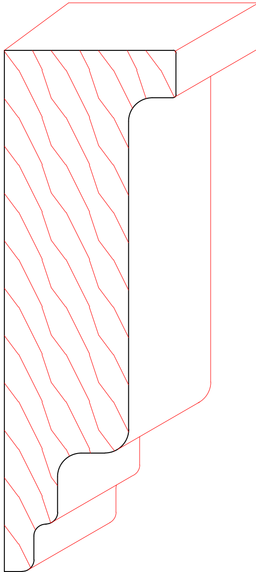
TM6052 1-13/16" x 5-1/2"
