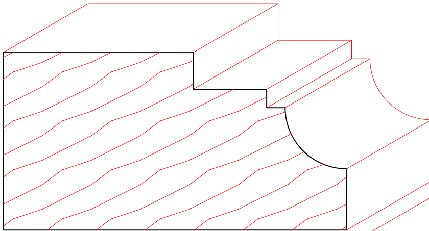
TM6016 1-3/4" X 3-1/2"
