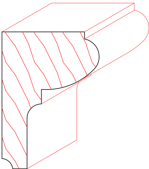
TM6060 1-11/16" X 2-3/8"
