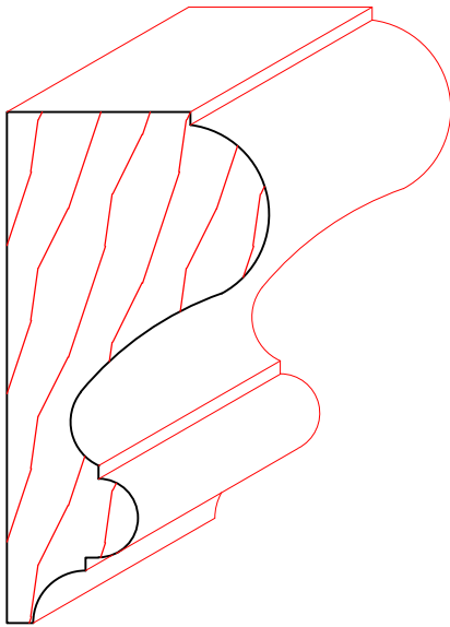
TM6062 1-1/4" X 2-7/16"
