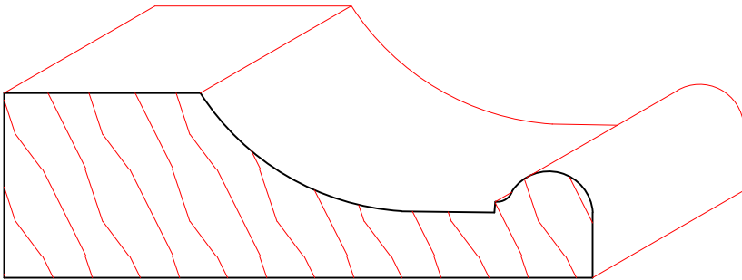
TM6029 1-1/16" X 3-3/8"
