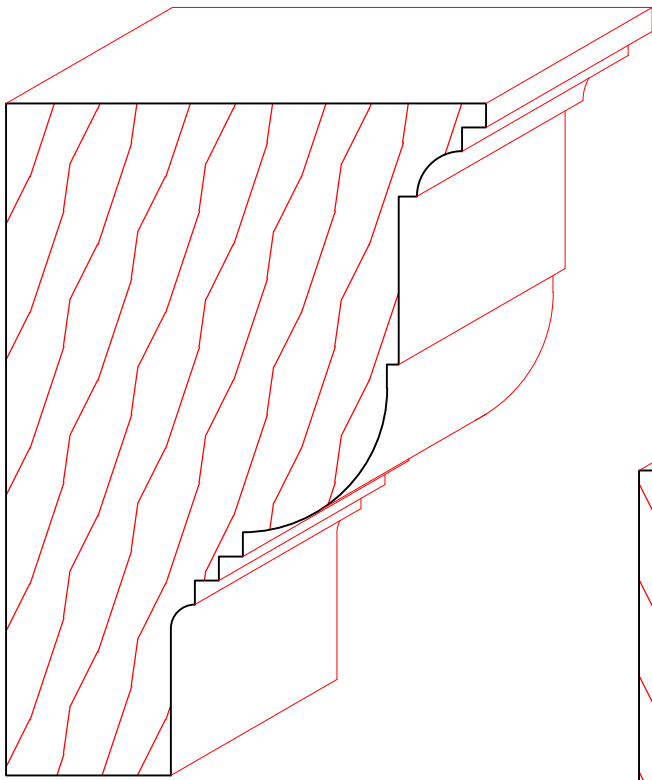
TM6073 2-1/2" X 3-1/2"
