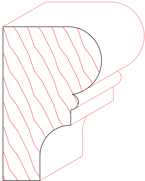
TM6072 2" X 3-1/8"
