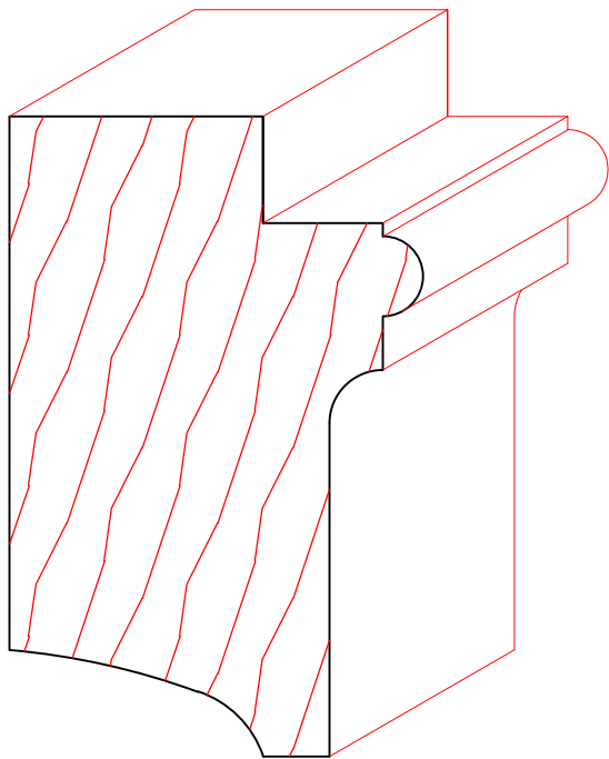
TM6058 1-15/16" X 3"
