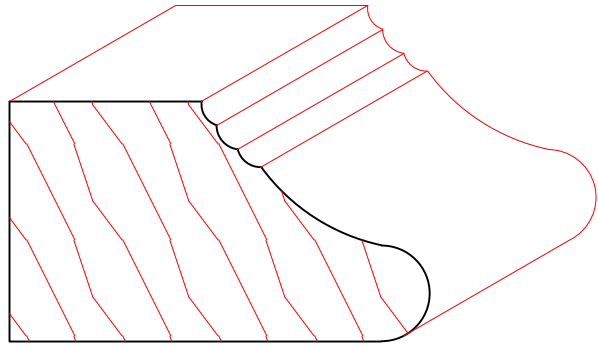
TM6011 1-1/4" X 2-3/16"
