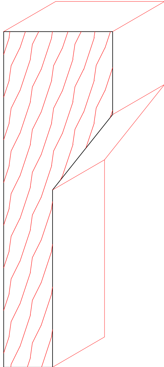
TM6065 1-13/16" X 5-9/16"
