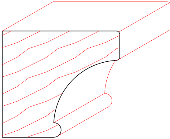
TM6051 1-13/16" x 2"
