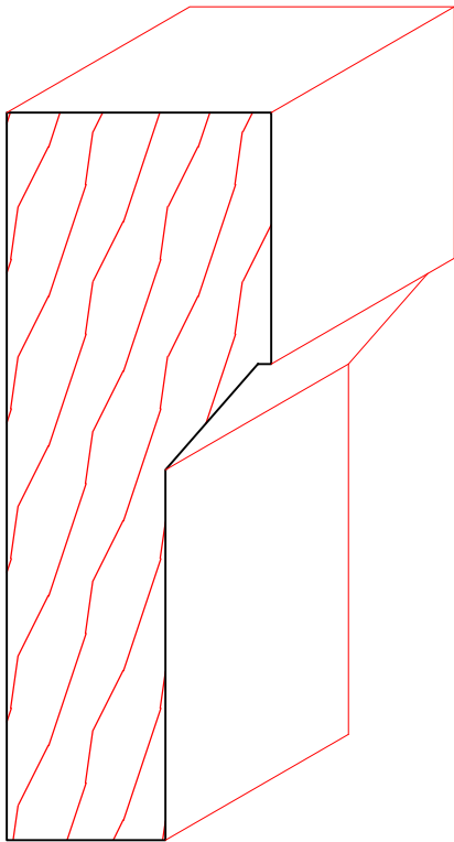
TM6077 1-1/4" X 3-7/16"
