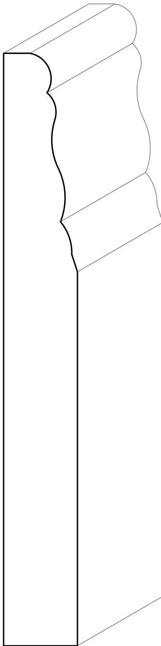
TM2164 3/4" X any width
