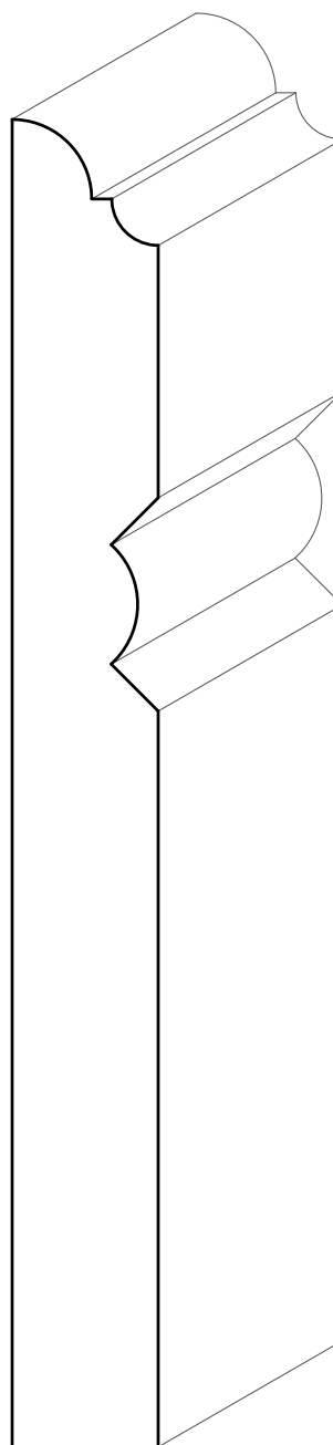
TM2035 11/16" X any width bead position can be adjusted
