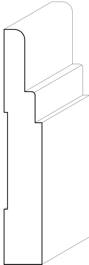
TM2032 3/4" X any width
