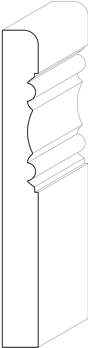
TM2242 5/8" X any width
