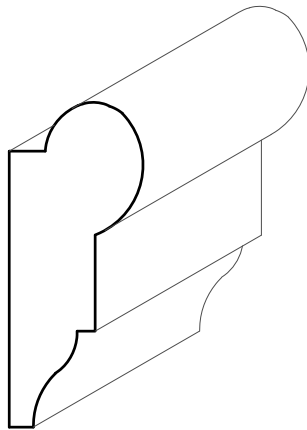
TM7024 \frac{11}{16}" \times 1\frac{11}{16}"
