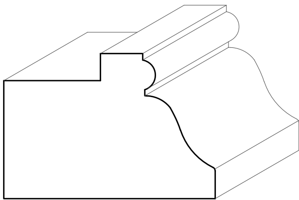
TM7408 1\frac{1}{2}" \times 2\frac{3}{16}"
