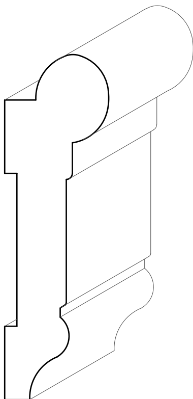
TM7027 1\frac{1}{16}" X 3\frac{1}{2}"
