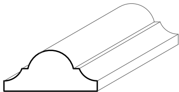
TM7307 \frac{7}{16}'' \times 1''
