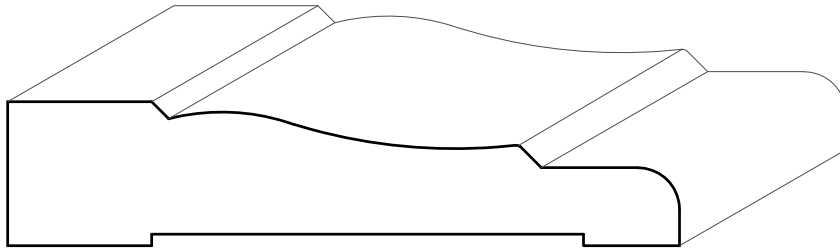
TM1352 3/4'' \times 3-1/2''
