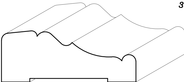
TM1166 15/16" X 2-3/8"
