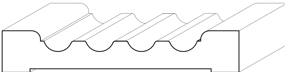
TM1091 3/4" \times 4-1/4"
