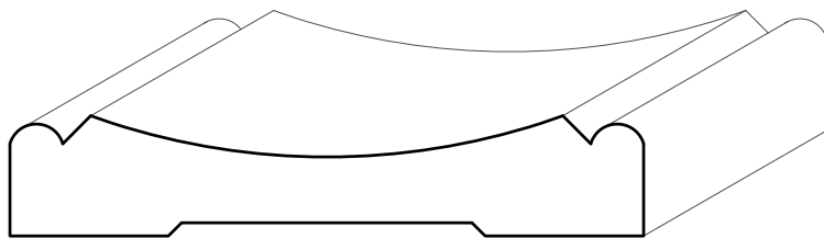
TM1007 9/16" X 3"
