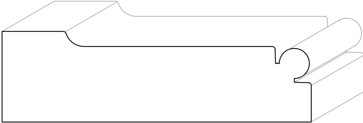
TM1241 1-1/2" X 5-1/8"
