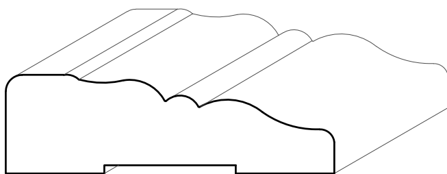
TM1120 3/4" X 2-1/2"
