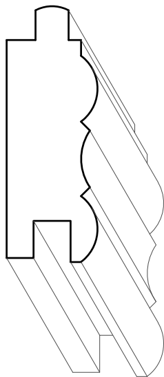
TM8002 11/16" X 1-15/16"
