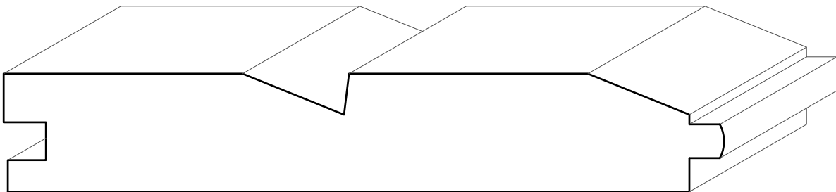
TM8047 7/8" X 5-5/16"
