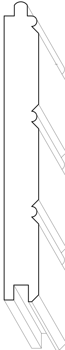
TM8133 5/8'' \times 5-3/8''
