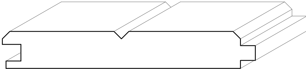
TM8074 3/4" X 5-1/16"
