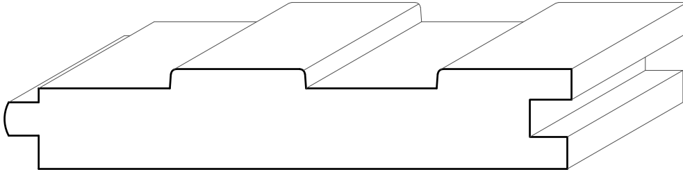
TM8119 3/4" X 4-1/4"
