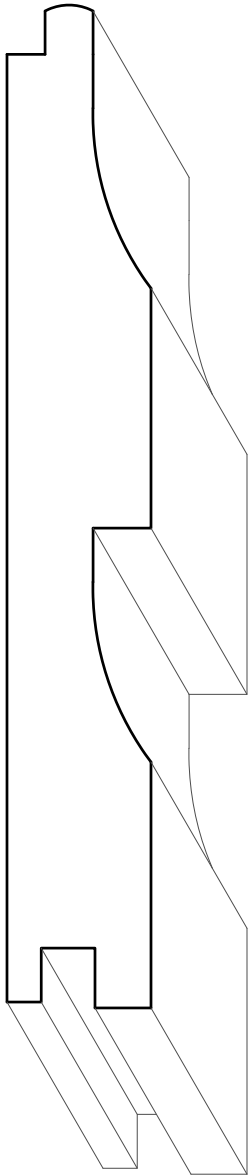
TM8007 3/4'' \times 5-3/16''+
