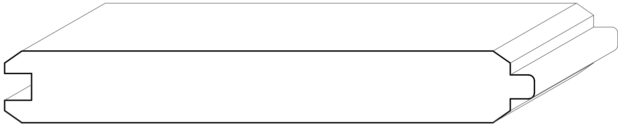
TM8041 3/4'' \times 5-1/2''
