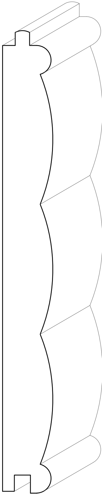
TM8056 7/8" X 8"
