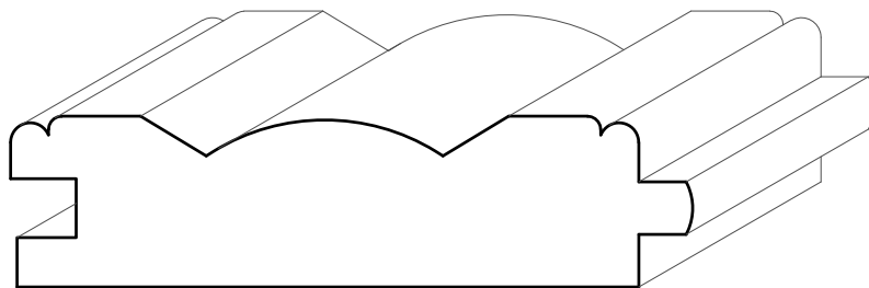
TM8042 13/16'' \times 3-1/4''
