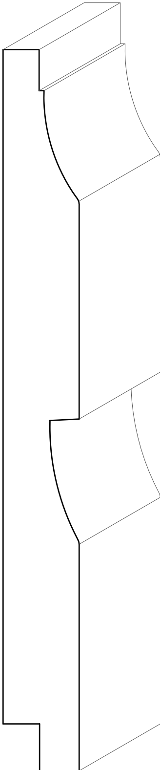
TM8076 13/16" X 7-11/16"
