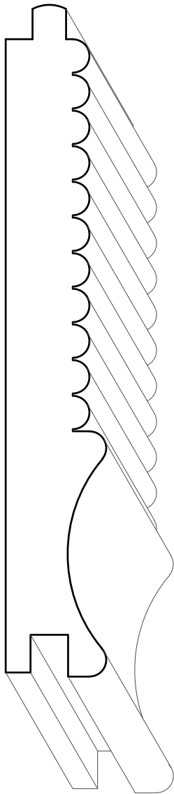
TM8018 3/4" X 5"
